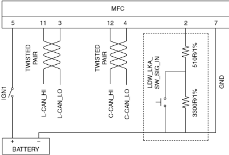
Connector A
