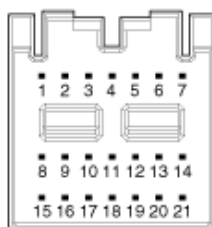
Connector C
