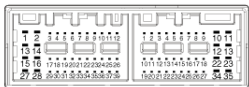
Connector A
