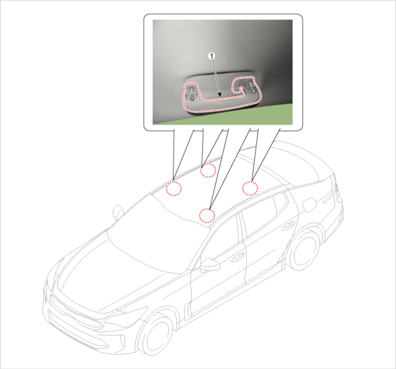
1. Assist handle
