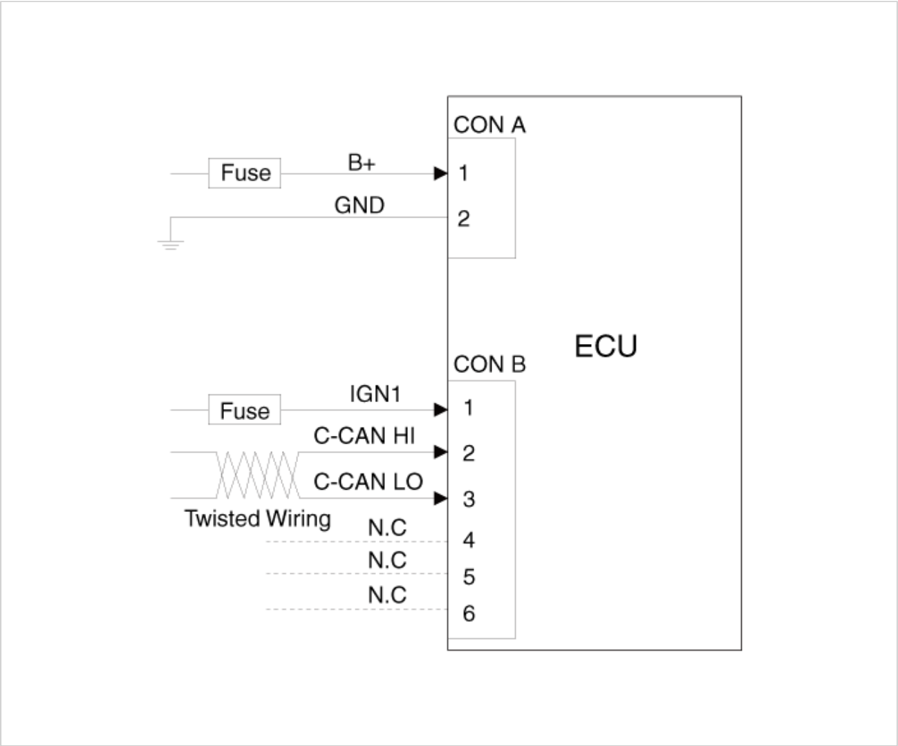
Harness Connector
