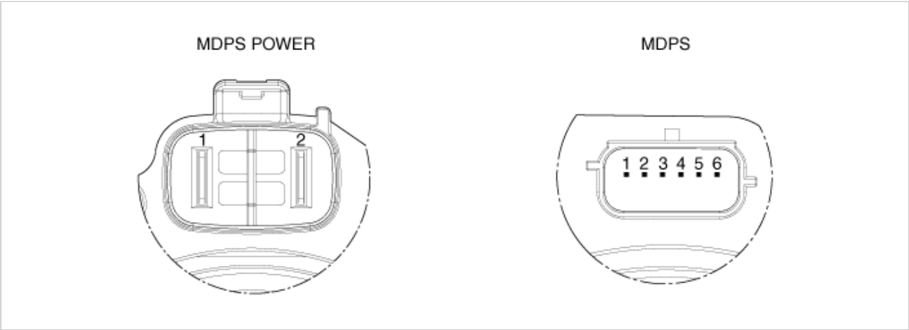
Harness Connector
