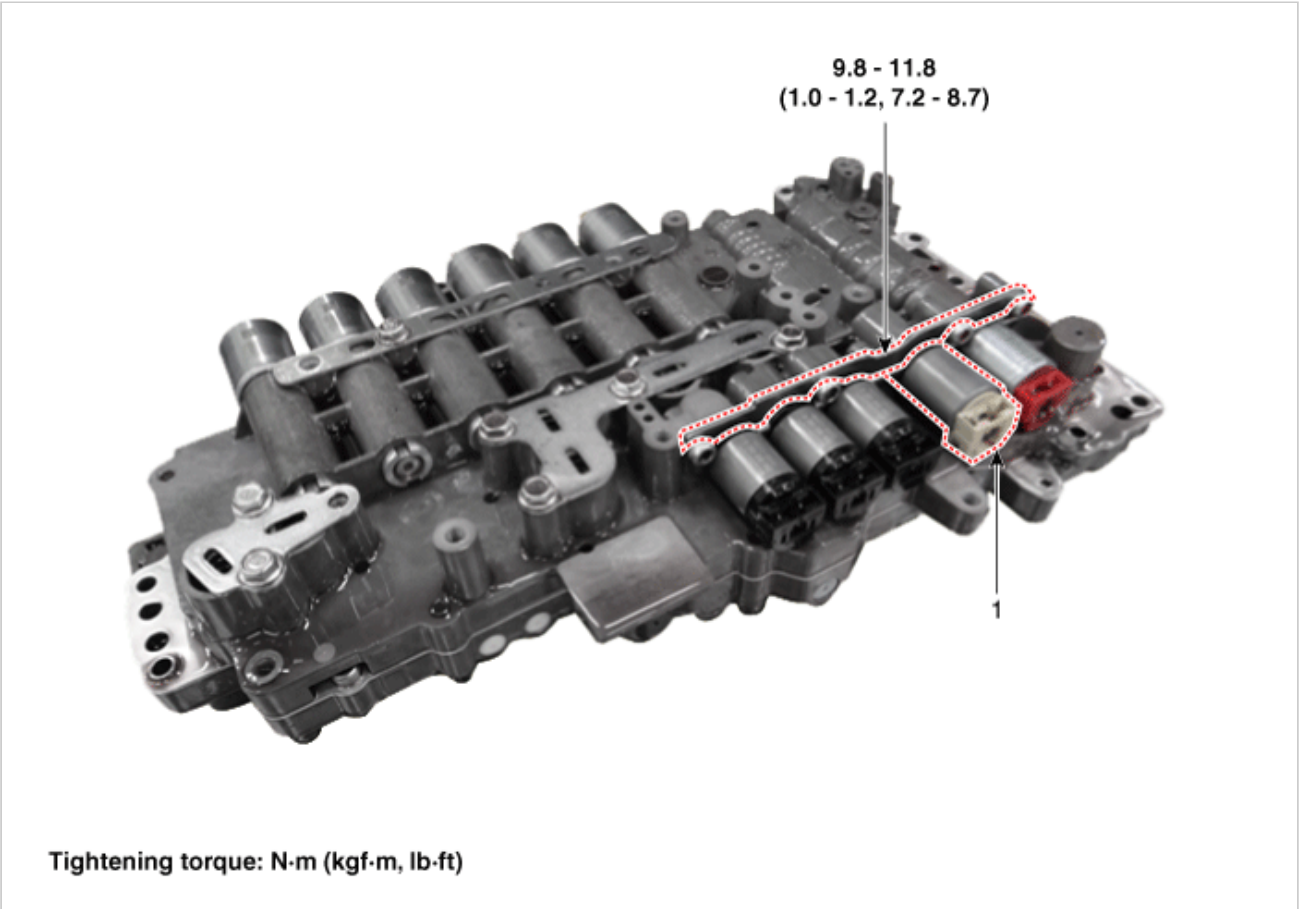
1. Damper clutch control solenoid valve Solenoid valve support bracket
