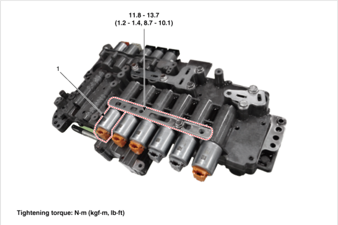
1. 8LR brake control solenoid valve
