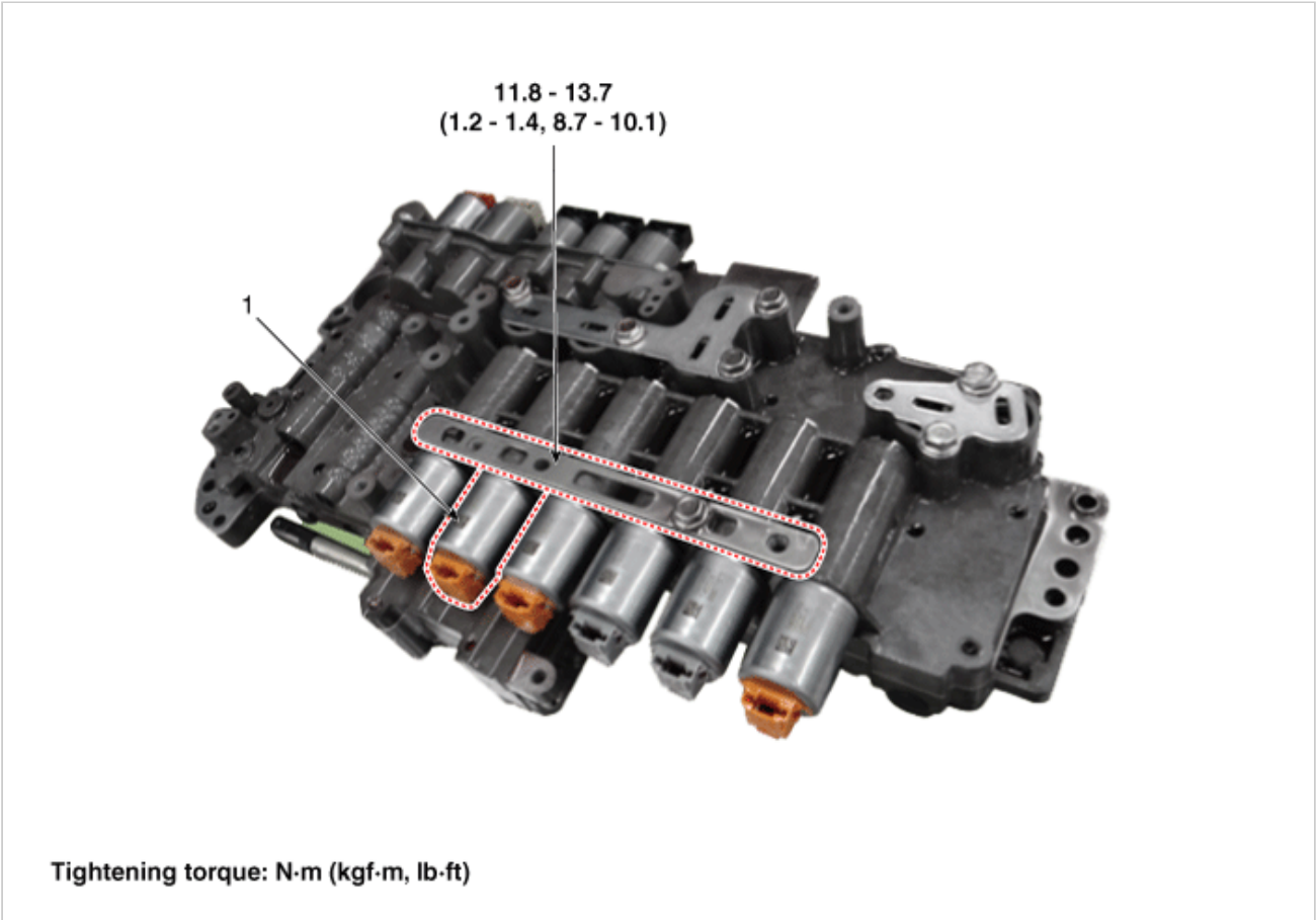
1. 6 clutch control solenoid valve
