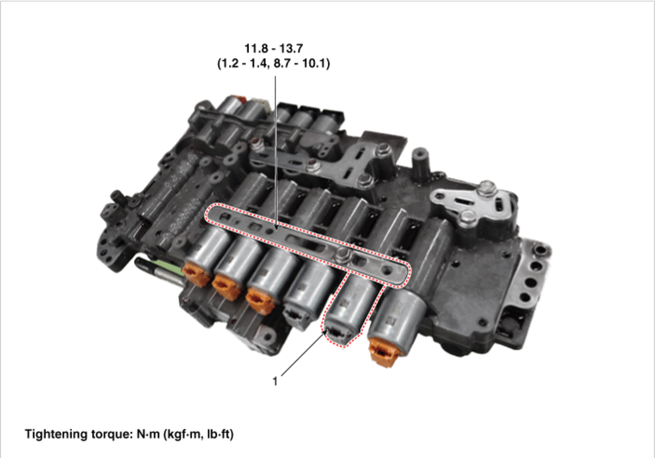
1. 4&OD clutch control solenoid valve 2. Solenoid valve support bracket
