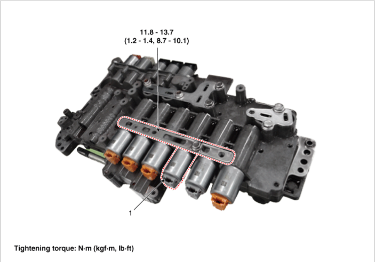
1. 35R clutch control solenoid valve 2. Solenoid valve support bracket
