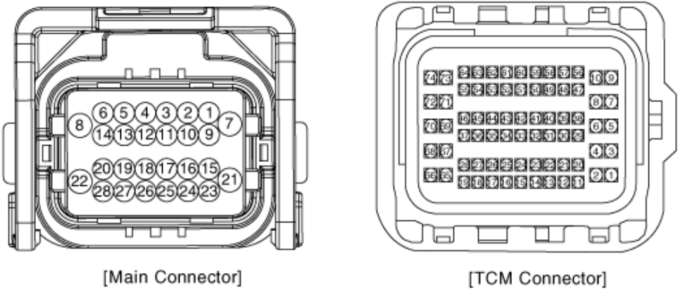
[Connector]
