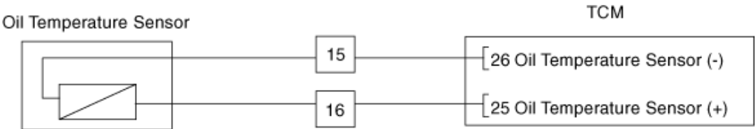
[Circuit Diagram]
