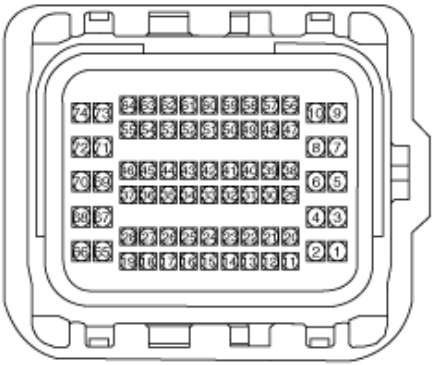
[TCM Connector]
