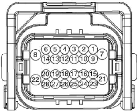
[Main Connector]
