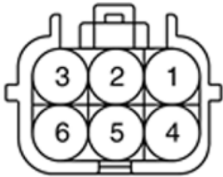
[Parking release actuator]
