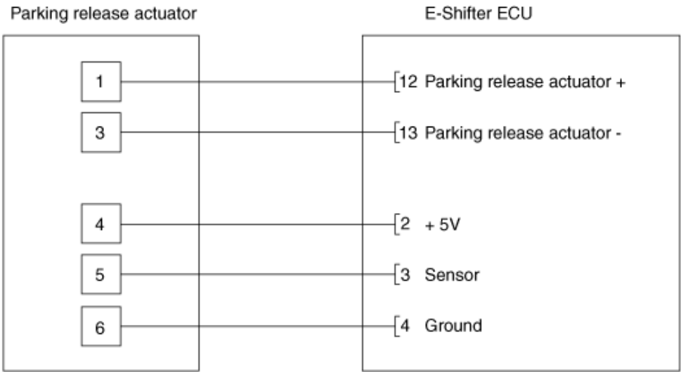
[Circuit Diagram]
