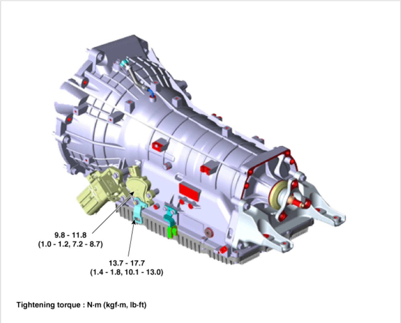
1. Inhibitor switch
