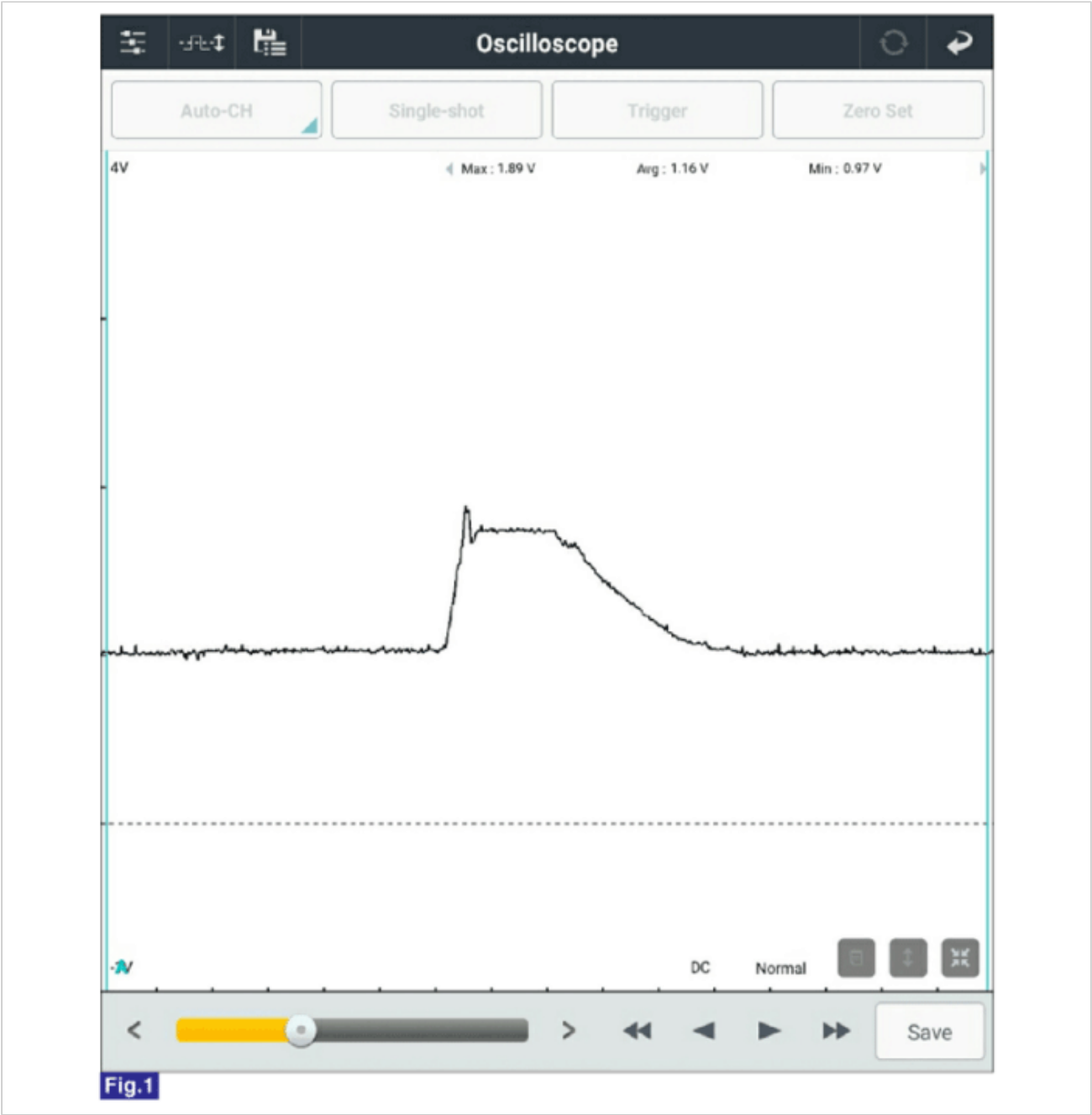
Fig.1) RPS waveform at acceleration.
