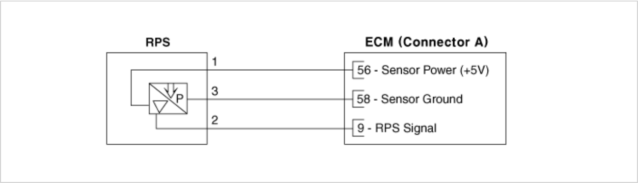
Harness Connector
