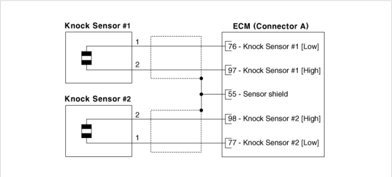
Harness Connector
