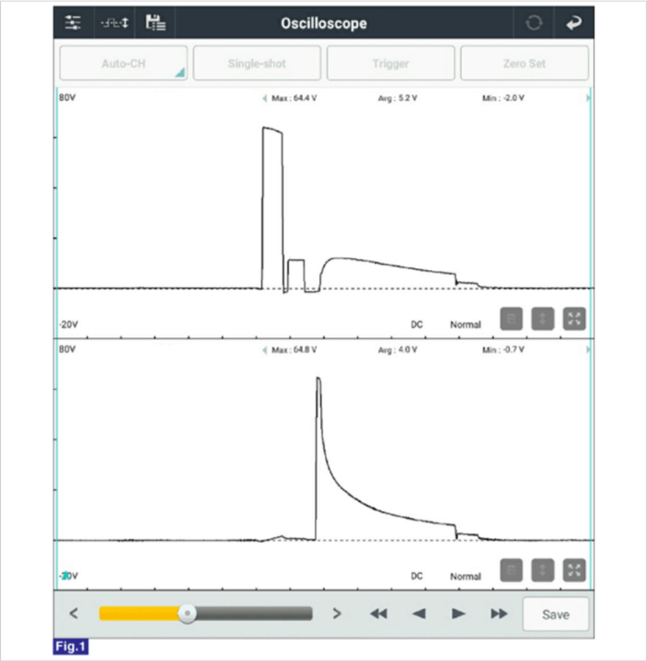
Fig.1) Normal Waveforms of Injector at Engine idle
