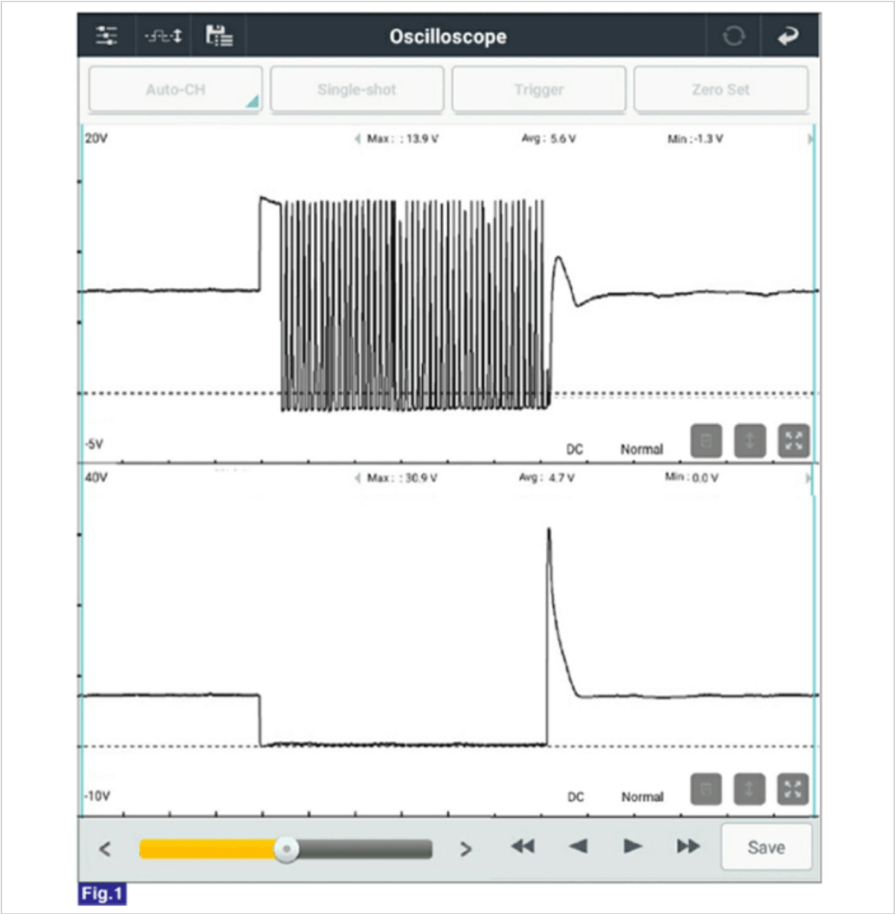
Fig.1) Normal Waveforms of FPCV at Engine idle.
