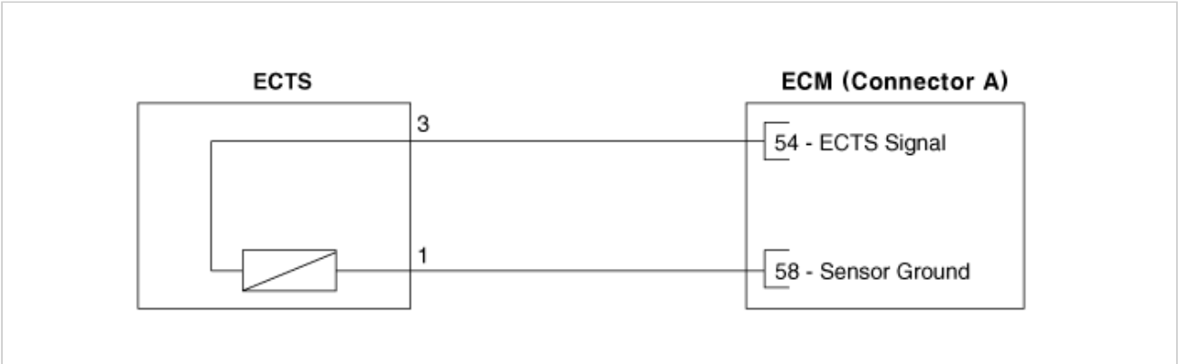
Harness Connector
