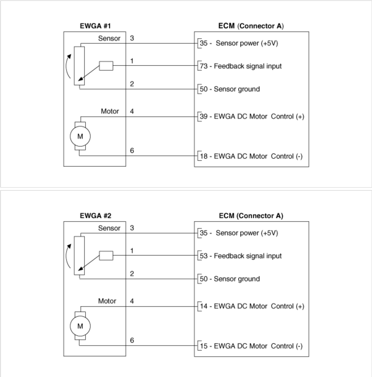
Harness Connector
