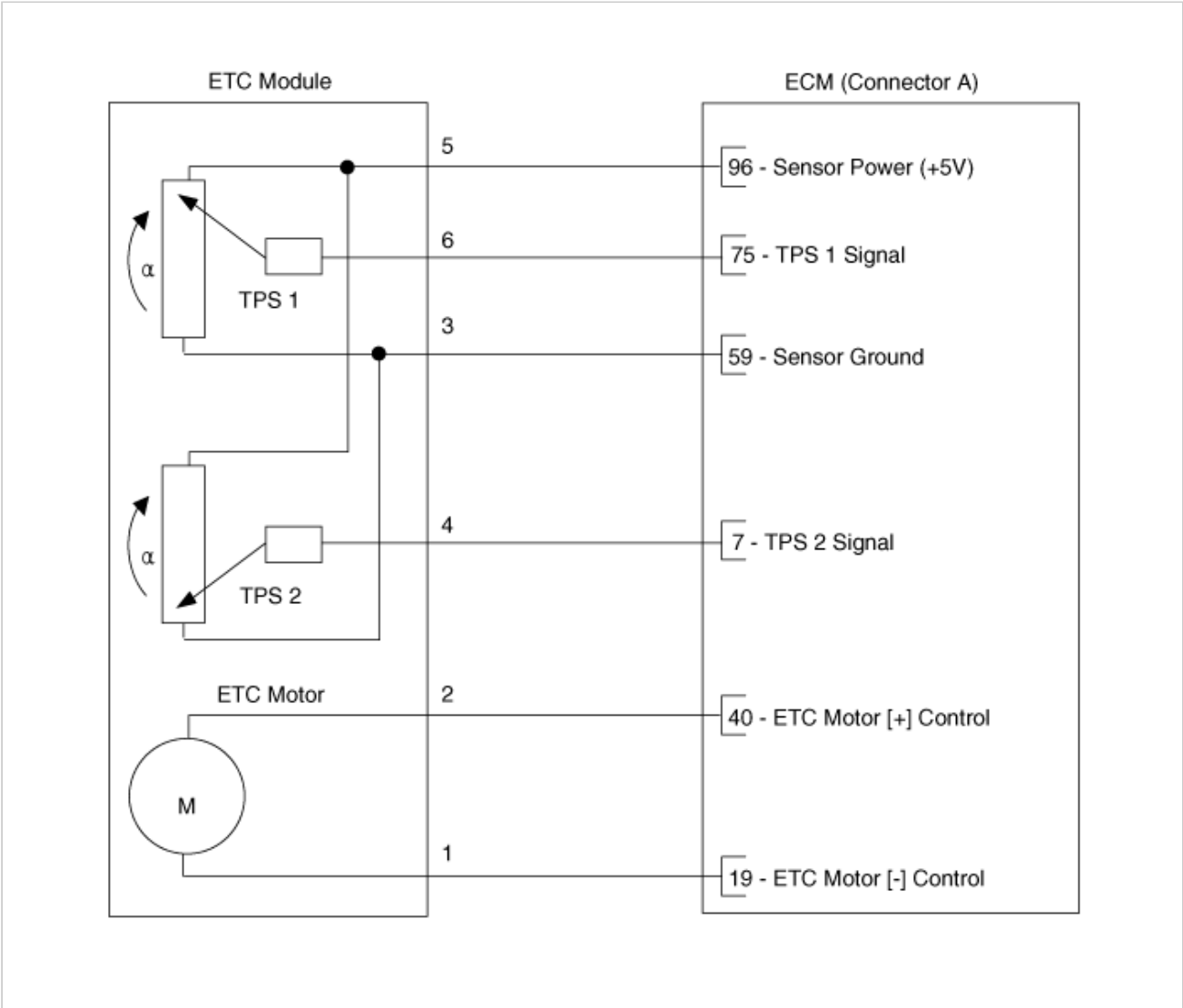
Harness Connector
