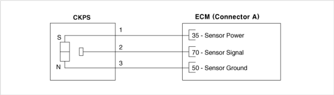
Harness Connector
