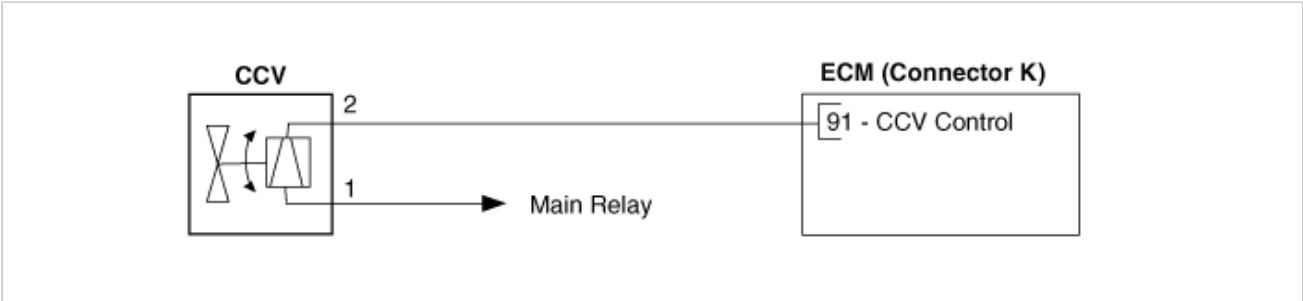
Harness Connector
