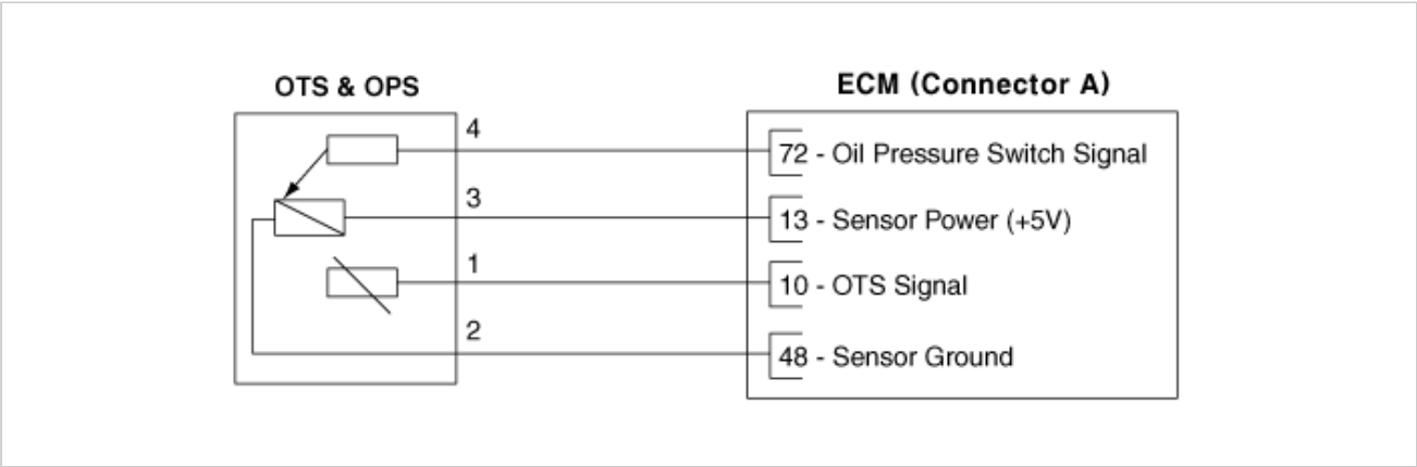
Harness Connector
